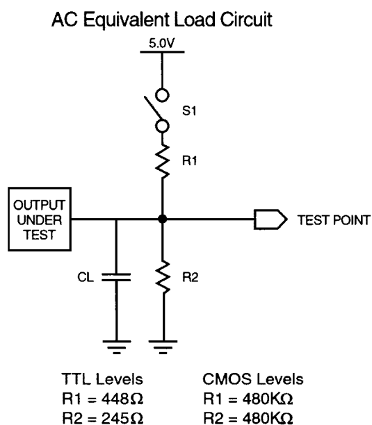
Figure 26: PEEL22CV10(Z) AC Test Loads/Waveforms
