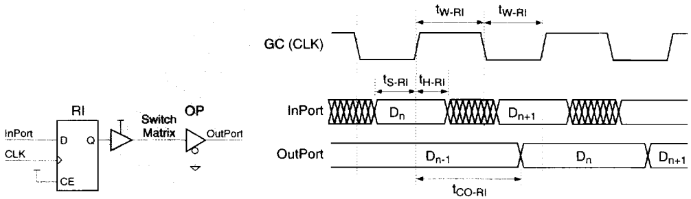
Timing Diagram 2: Registered Input Mode Timing
