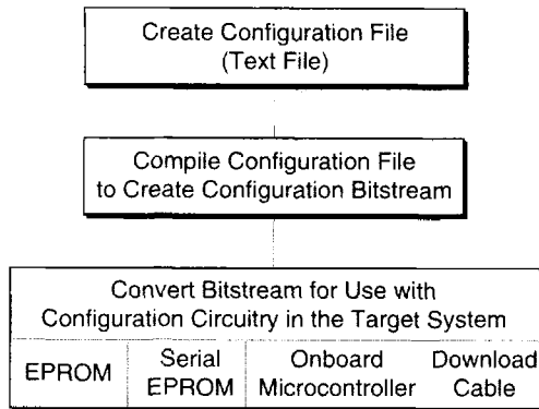
Figure 9: Off-line Bit Stream Generation
