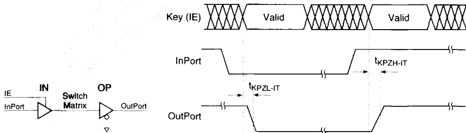
Timing Diagram 11:Key Timing for Input Enable
