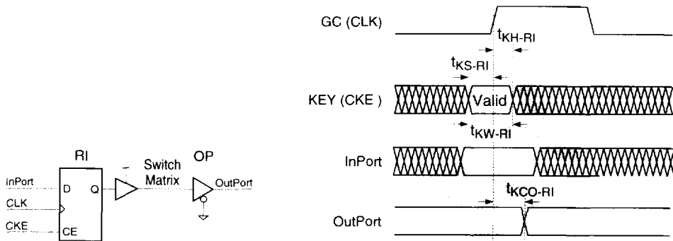
Timing Diagram 9:Key Timing for Register Input, Clock Enable (CKE)
