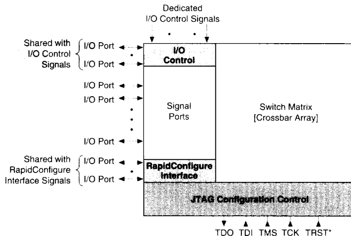
Figure 1: IQX Functional Block Diagram
