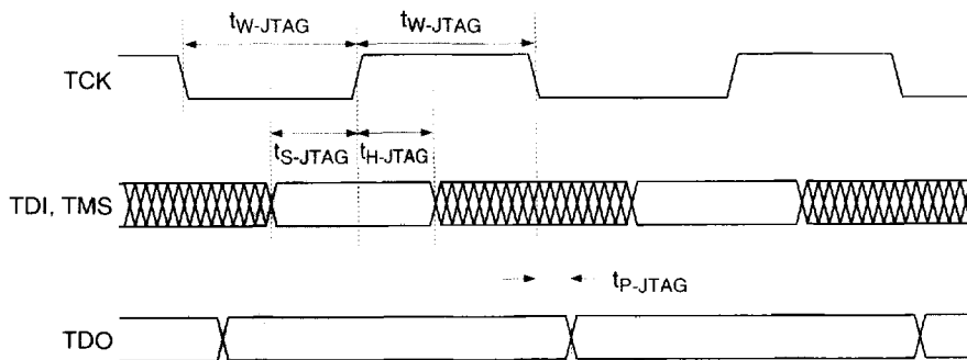
Timing Diagram 17: JTAG Timing
