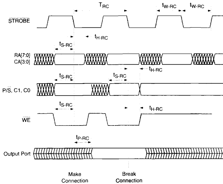
Timing Diagram 16: RapidConfigure Timing
