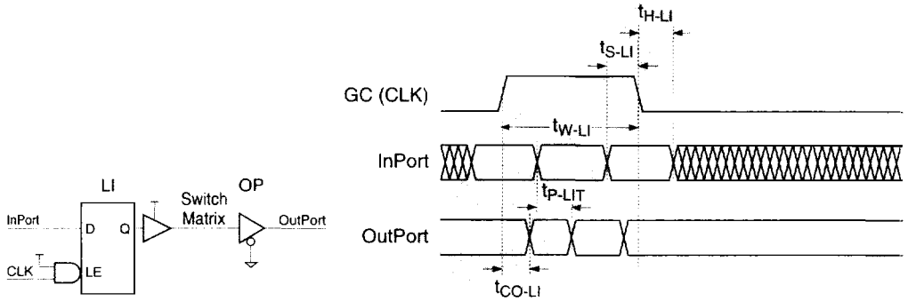
Timing Diagram 7: Latched Input Mode Timing
