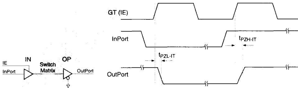
Timing Diagram 5: Input Enable Timing (Flow-through Mode)
