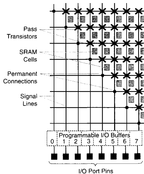
Figure 2: Switch Matrix Structure
