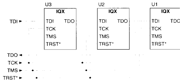
Figure 11: Configuring Multiple IQX Devices
