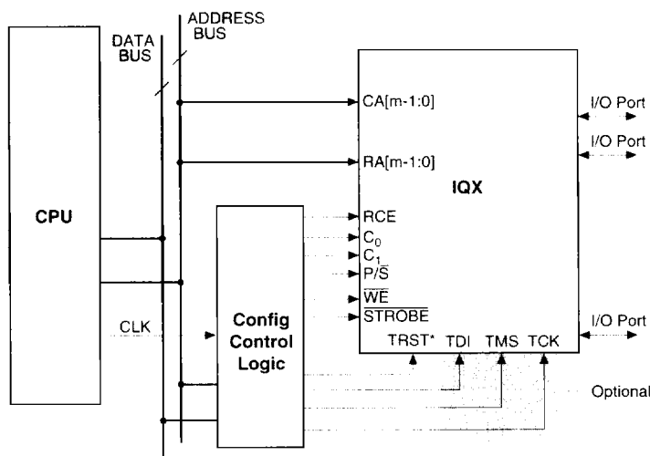
Figure 7: IQX RapidConfigure System Interface
