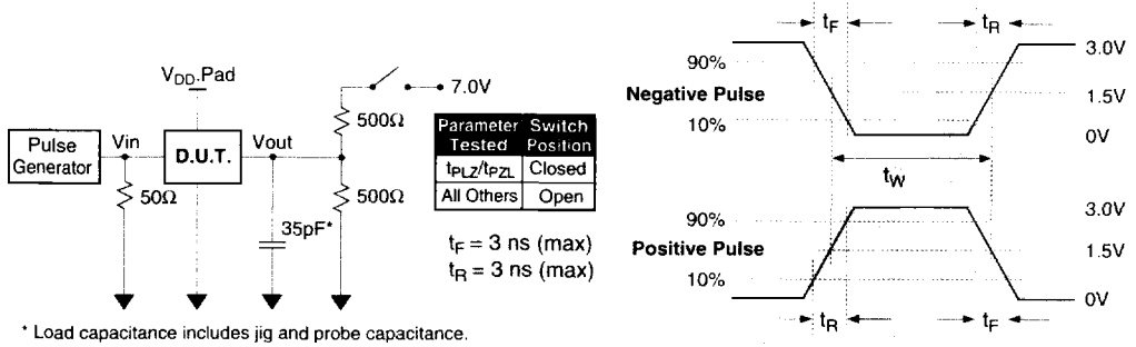
Figure 15: Test Circuit and Waveform Definition
