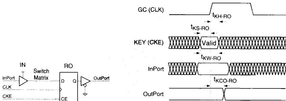
Timing Diagram 10:Key Timing for Register Output, Clock Enable (CKE)
