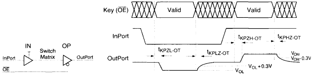
Timing Diagram 12:Key Timing for Output Enable
