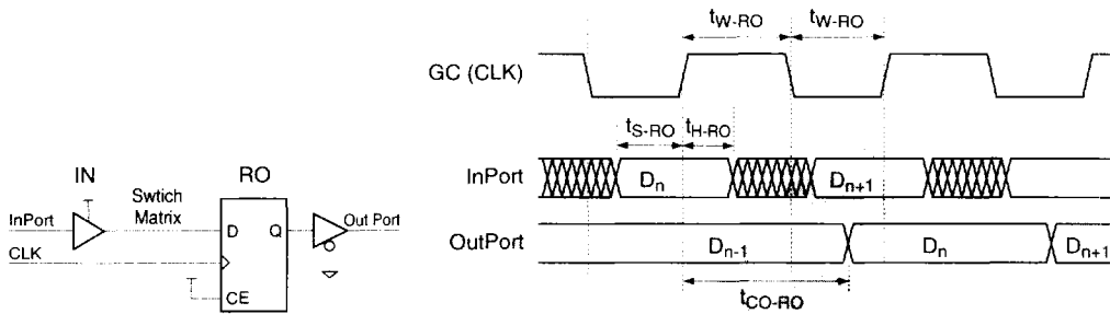
Timing Diagram 3: Registered Output Mode Timing
