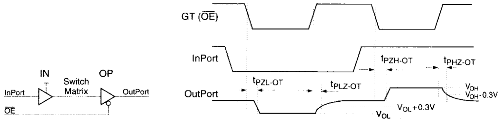
Timing Diagram 6: Output Enable Timing (Flow-through Mode)
