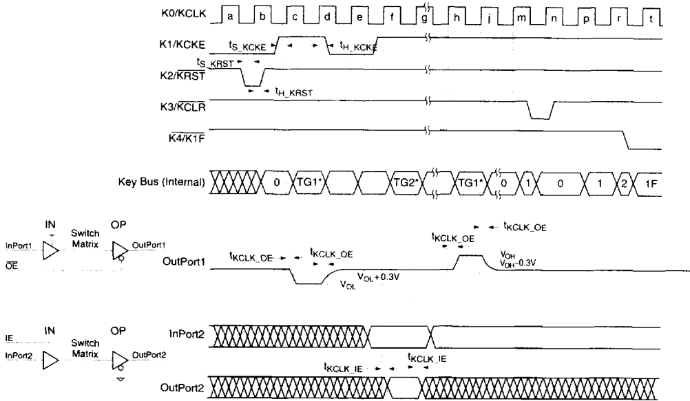
Timing Diagram 15: Key Counter Timing
