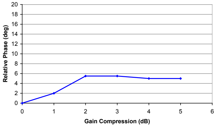
XP1006, Phase (degrees) vs Gain Compression (dB)
