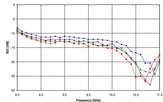
Output return loss ( V_d=8V , V_{gg}=-5V )
