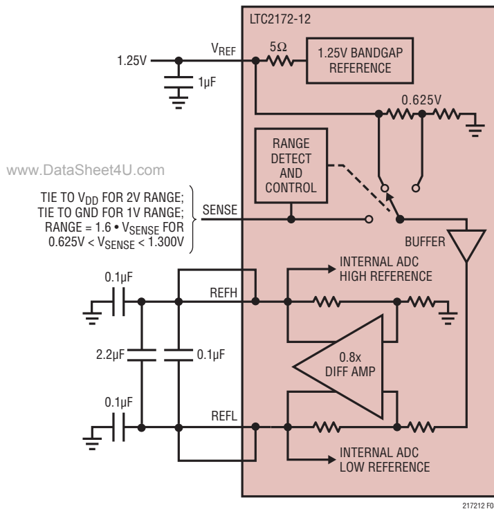
Figure 8. Reference Circuit
