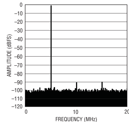
LTC2171-12: 8k Point FFT, f_{IN} = 5\text{MHz} , -1dBFS, 40Mps
