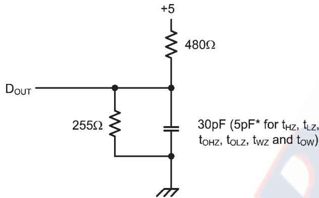
Figure 1. Output Load
