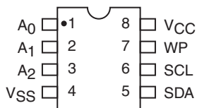
DIP Package (P)
