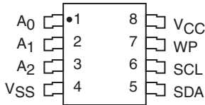
MSOP Package (R)
