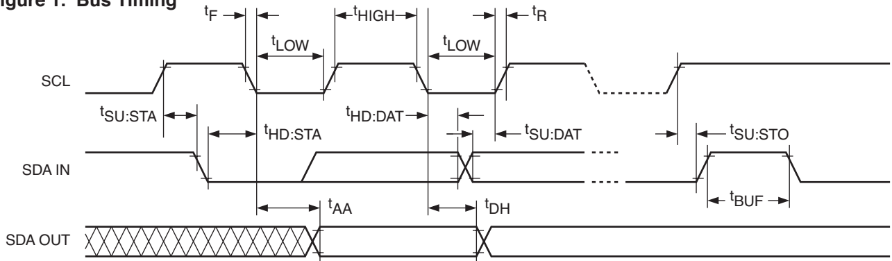
Figure 1. Bus Timing
