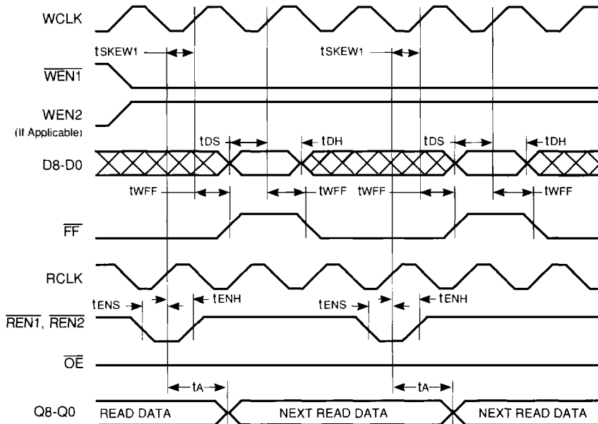
FIGURE 9. FULL FLAG TIMING
