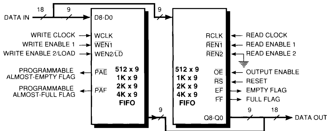
FIGURE 16. WIDTH-EXPANSION MODE
