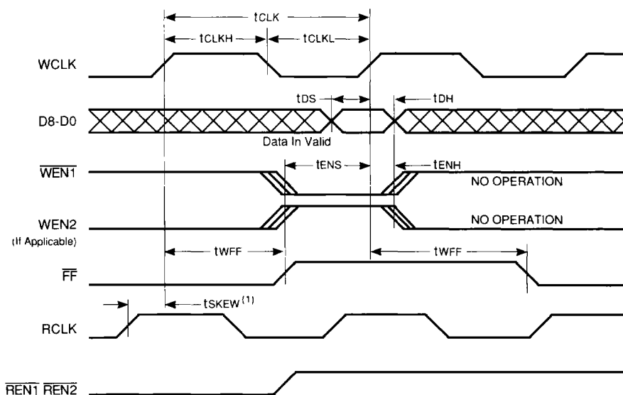
FIGURE 5. WRITE CYCLE TIMING
