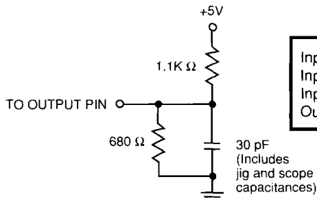
FIGURE 3. AC TEST CONDITIONS
