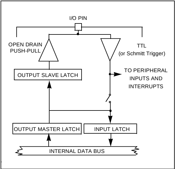
Figure 52. Output Configuration
