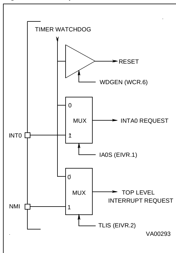
Figure 57. Interrupt Sources
