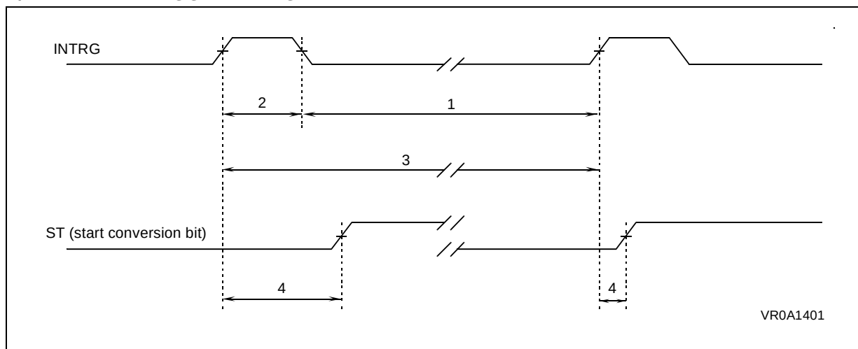
A/D INTERNAL TRIGGER TIMING
