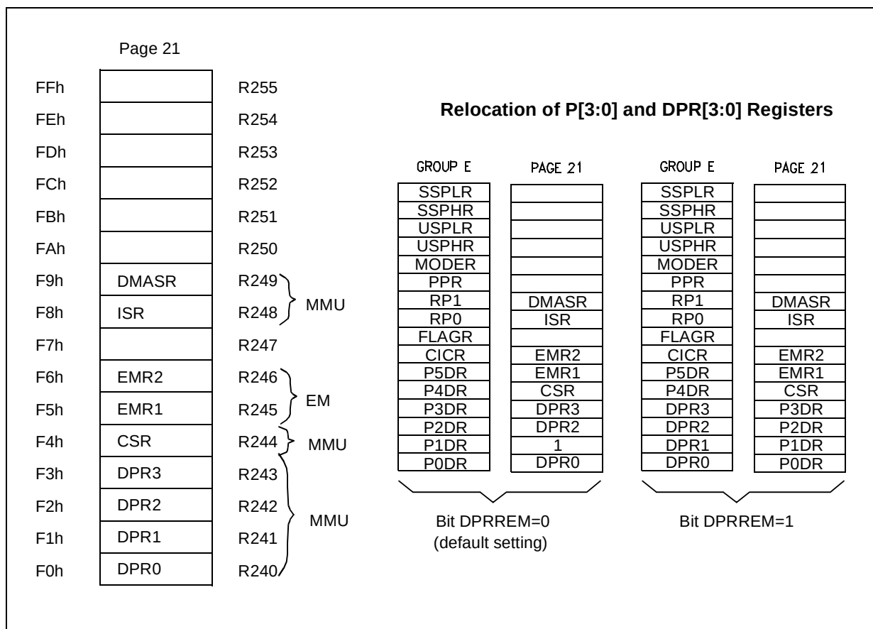
Figure 13. Page 21 Registers
