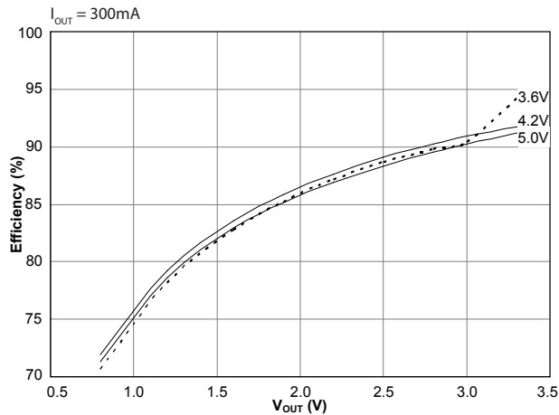
Efficiency vs. V_{OUT} ( T_A = 85^\circ C )
