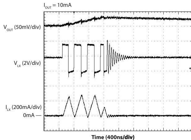
Light Load Switching — V_{OUT} = 1.8V
