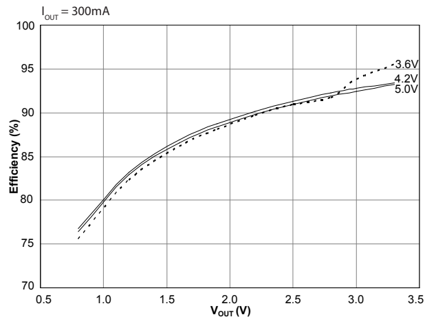
Efficiency vs. V_{OUT} ( T_A = -40^\circ C )
