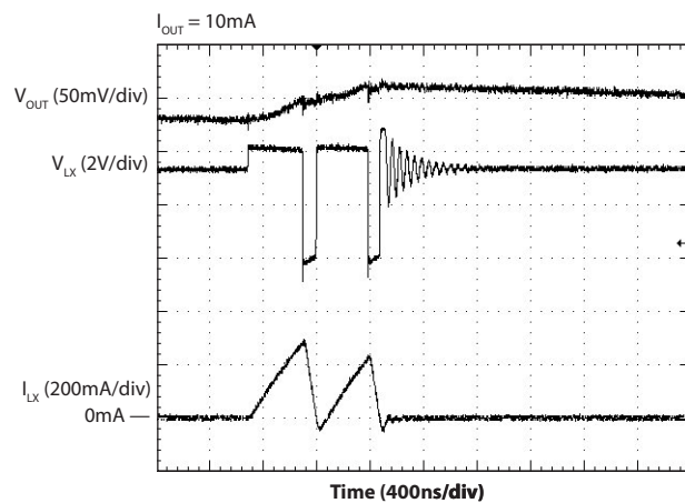
Light Load Switching — V_{OUT} = 3.3V
