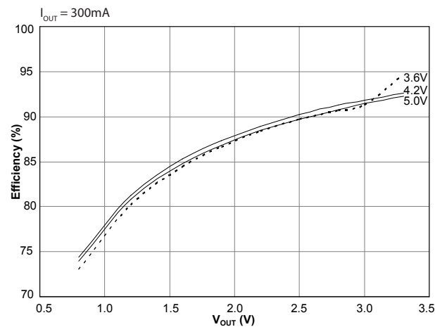
Efficiency vs. V_{OUT} ( T_A = 25^\circ C )
