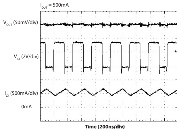
Heavy Load Switching — V_{OUT} = 1.8V
