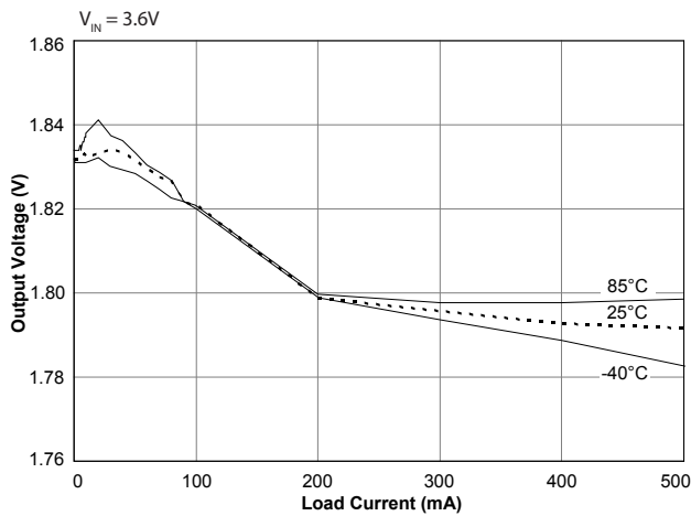
Load Regulation ( V_{OUT} = 1.8V )
