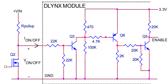
Figure 40. Circuit configuration for using negative On/Off logic.
