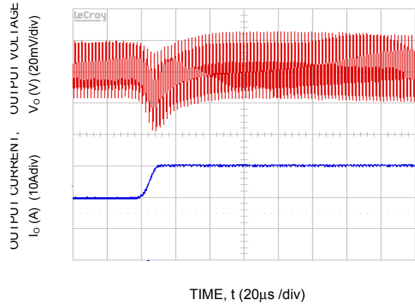
Figure 10. Transient Response to Dynamic Load Change from 50% to 100% at 12Vin, C_{out}= 1x47\mu F +5x330\mu F . C_{Tune}=10nF & R_{Tune}=178 ohms
