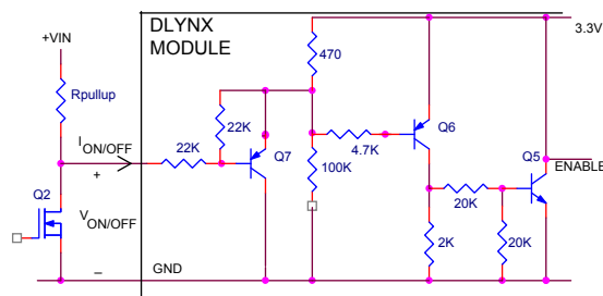
Figure 39. Circuit configuration for using positive On/Off logic.
