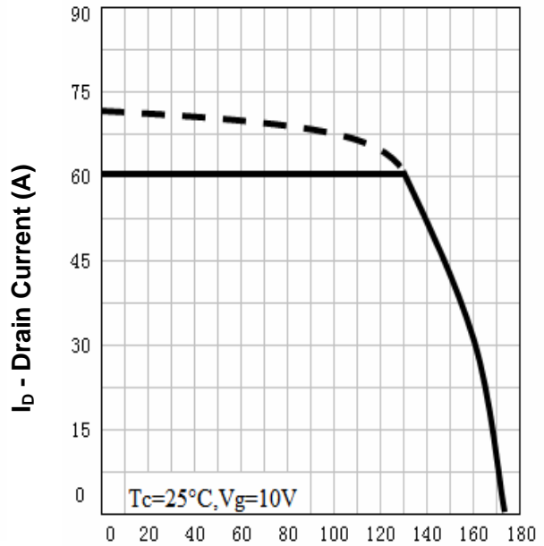
Drain Current
