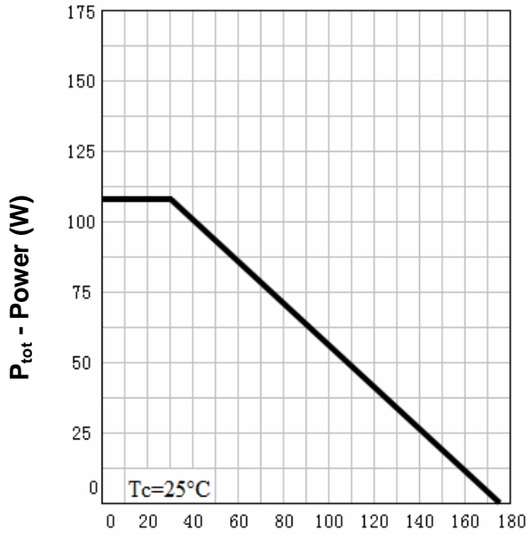
Power Dissipation
