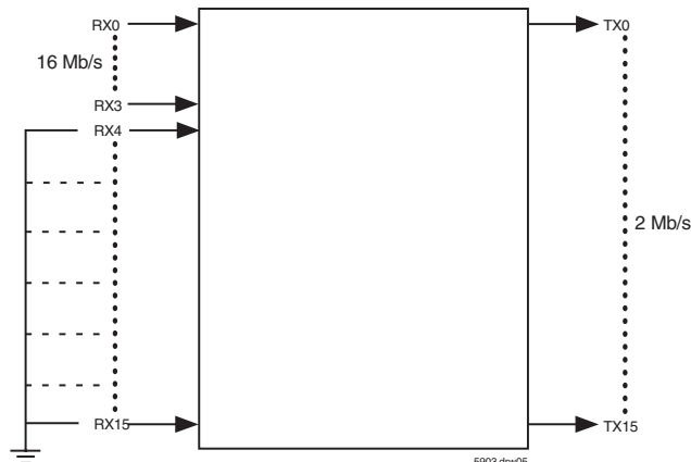
Figure 4. Mux/Demux Mode
