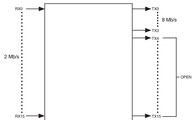
Figure 4. Mux/Demux Mode
