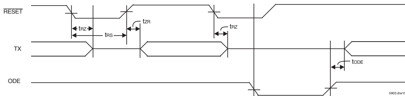
Figure 8. Reset and ODE Timing
