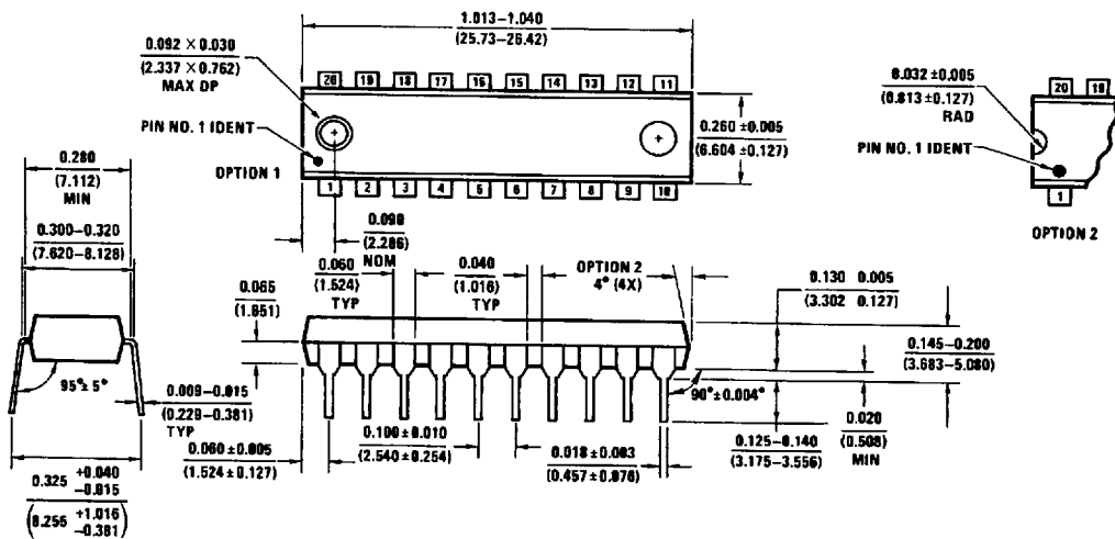
Molded Dual-In-Line Package (N) Order Number DM74AS240N or DM74AS244N NS Package Number N20A
