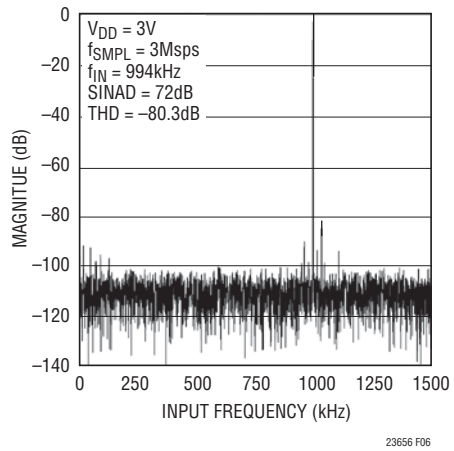
Figure 6. LTC2366 FFT Plot
