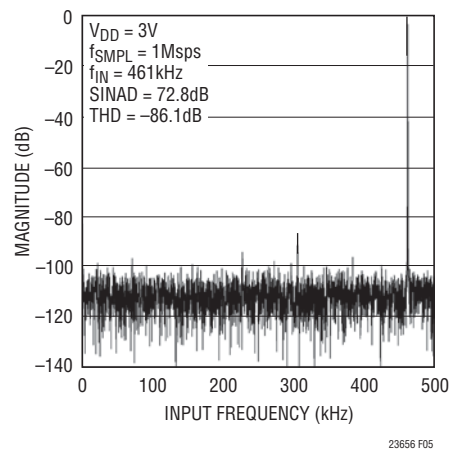
Figure 5. LTC2365 FFT Plot
