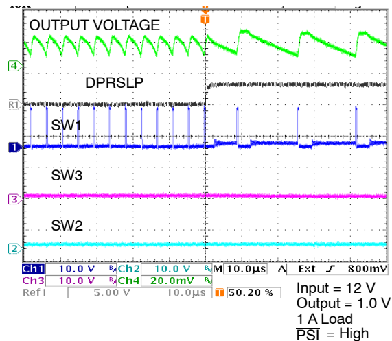
Figure 21. DPRSLP Transition
