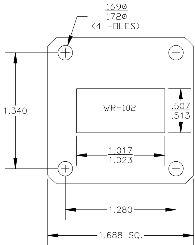
BACK VIEW
