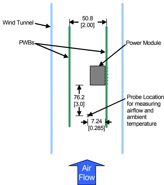
Figure 44. Thermal Test Set-up.
