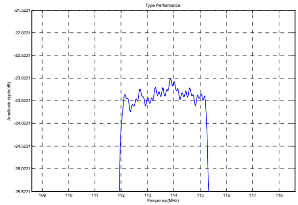
Passband Respond
