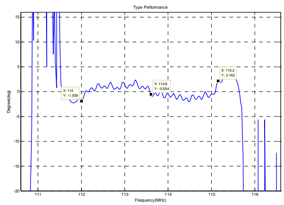
Phase Linearity( f_0 \pm 1.6 MHz)
