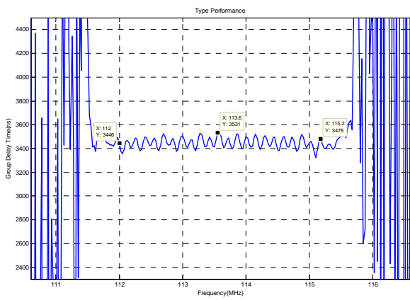
Group Delay Variation( f_0 \pm 1.6 MHz)
