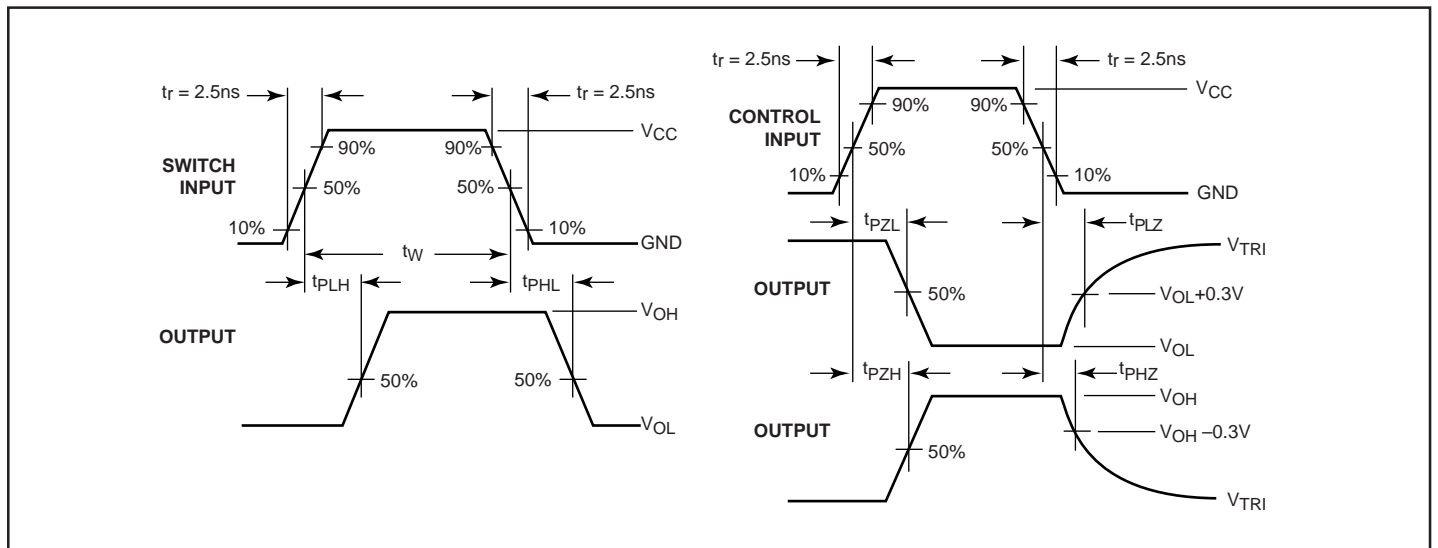
Figure 2. AC Waveforms
