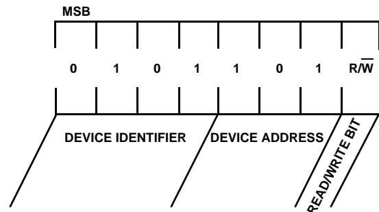
FIGURE 27. SLAVE ADDRESS BYTE DEFINITION
