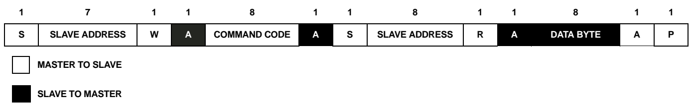
FIGURE 30. READ BYTE PROTOCOL for ISL97694A
