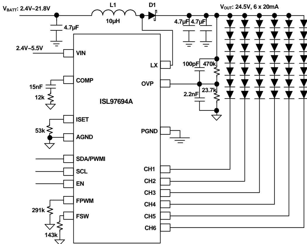
FIGURE 26. LED DRIVER OPERATION WITH INPUT VOLTAGE UP TO 26V
