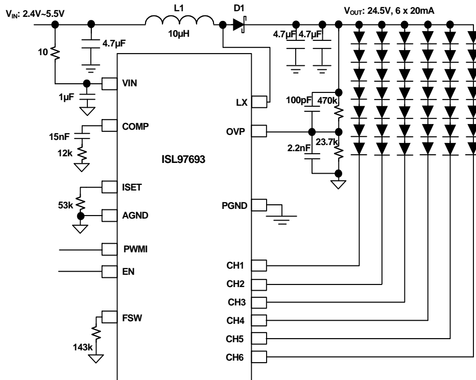
FIGURE 4. ISL97693 TYPICAL APPLICATION DIAGRAM
