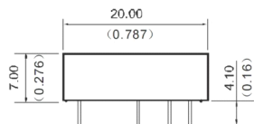
IF-XD-1W DIP
