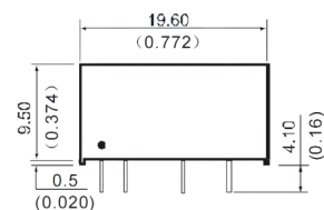
IF-XS-1W SIP
