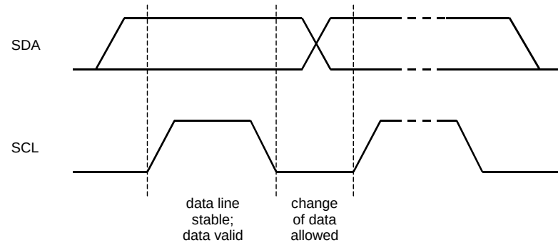
Figure 58. Bit Transfer on the I 2 C-Bus
