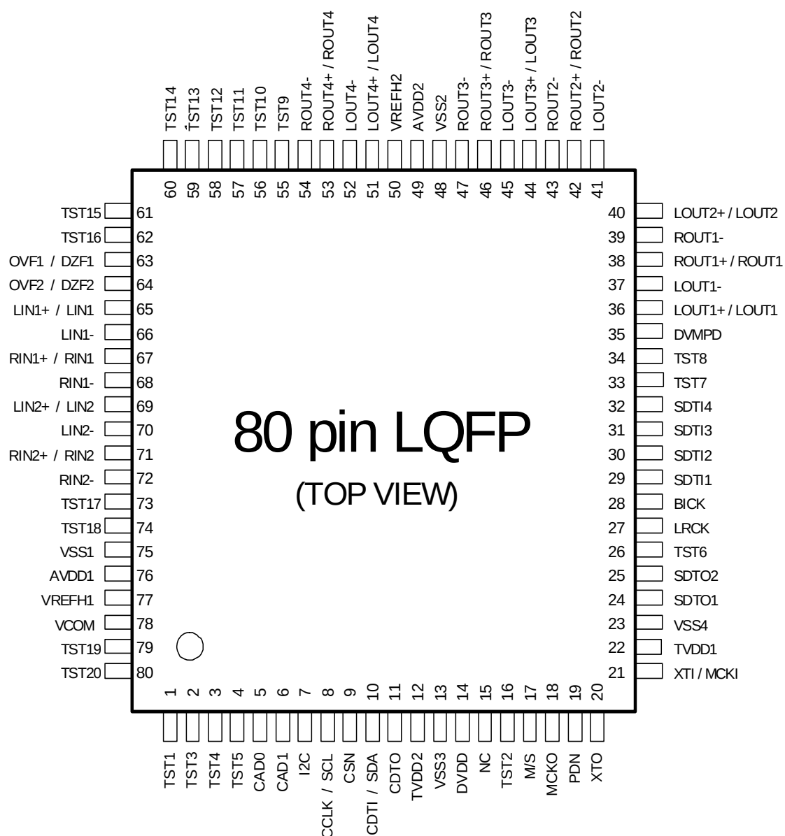
Figure 2. Pin Layout
