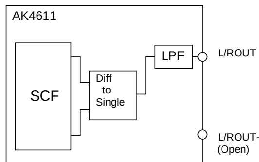
Figure 22. Single-end Output (DOE1-4 bit = “0”)
