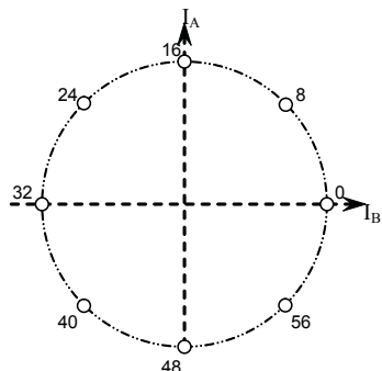
Figure 8. Half-step phase diagram using STEP input
