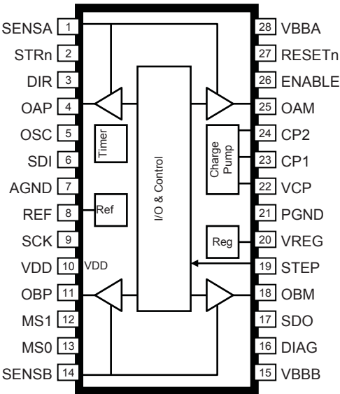
Pin-out Diagram
