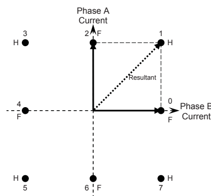
Figure A4. Phase diagram for simple half step
