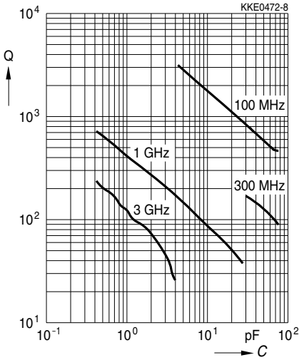
Q factor versus capacitance C
