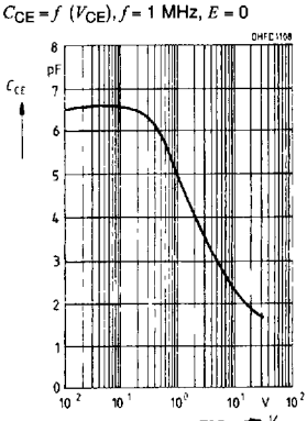
Collector-emitter capacitance
