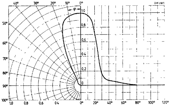
Directional characteristics S_{rel} = f(\varphi)
