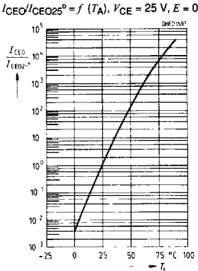
Dark current
