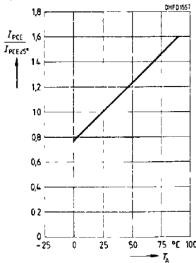
Photocurrent I_{PCE}/I_{PCE25^\circ} = f(T_A), V_{CE} = 5 \text{ V}
