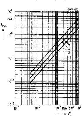
Photocurrent I_{PCE} = f(E_\theta), V_{CE} = 5 \text{ V}
