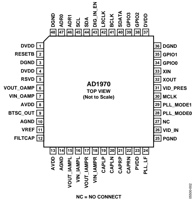
Figure 2. Pin Configuration
