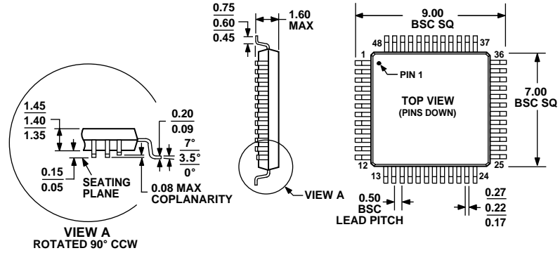
Figure 9. 48-Lead Low-Profile Quad Flat Package [LQFP] (ST-48)
