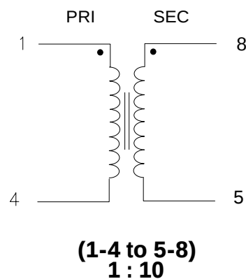
Schematic Diagram
