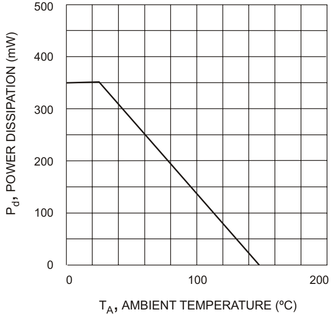
Fig. 4 Power Dissipation Derating
