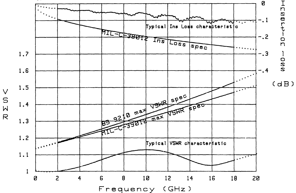
Typical VSWR/Insertion loss plot for SMA mated pair on RG 405 (0.085")
