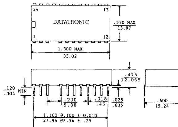
PACKAGE: DIP
