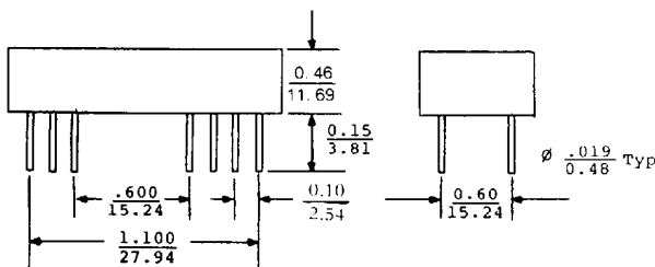
PACKAGE: DIL
