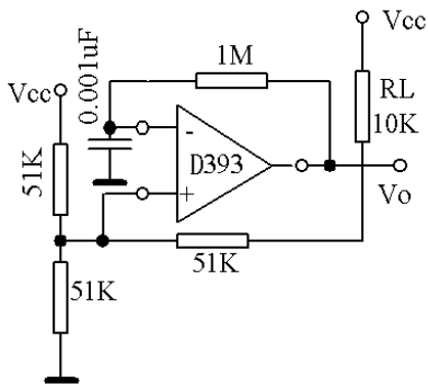
Applied single power Supply
