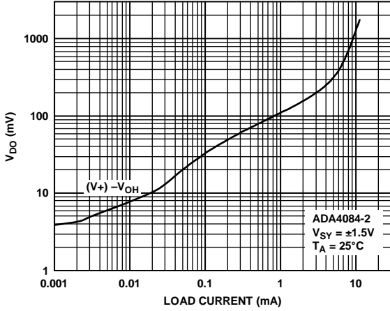
Figure 9. Dropout Voltage vs. Source Current
