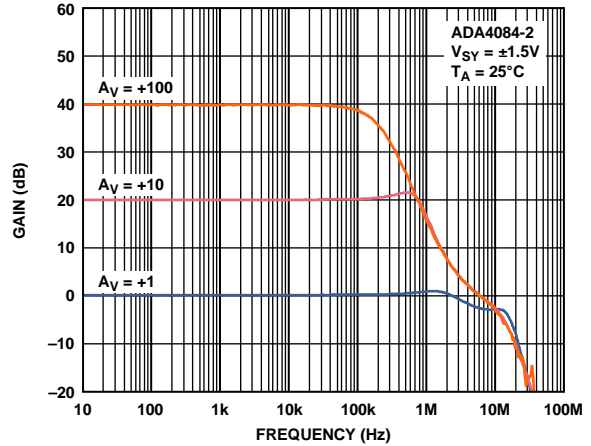
Figure 12. Closed-Loop Gain vs. Frequency
