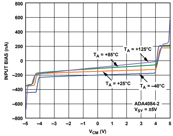
Figure 31. Input Bias Current vs. V CM and Temperature
