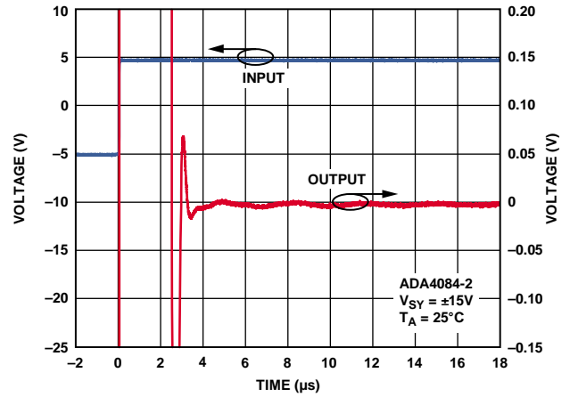
Figure 64. Settling Time
