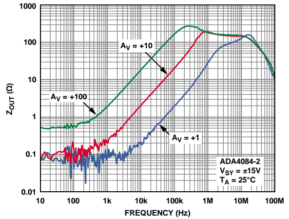
Figure 59. Output Impedance vs. Frequency
