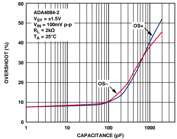
Figure 20. Overshoot vs. Capacitance
