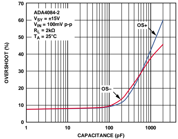
Figure 66. Overshoot vs. Load Capacitance
