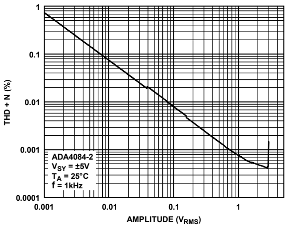
Figure 46. THD + N vs. Amplitude
