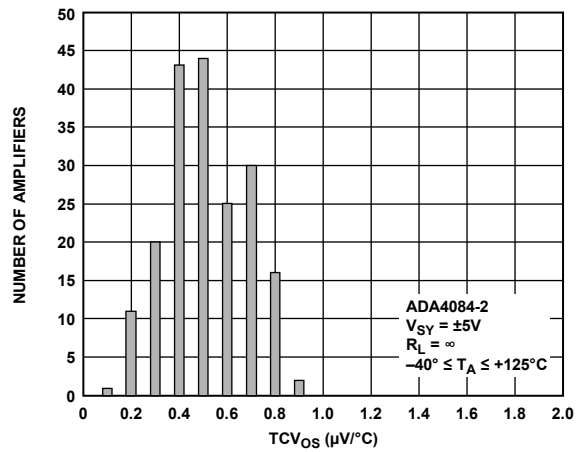
Figure 28. TCV 0s Distribution
