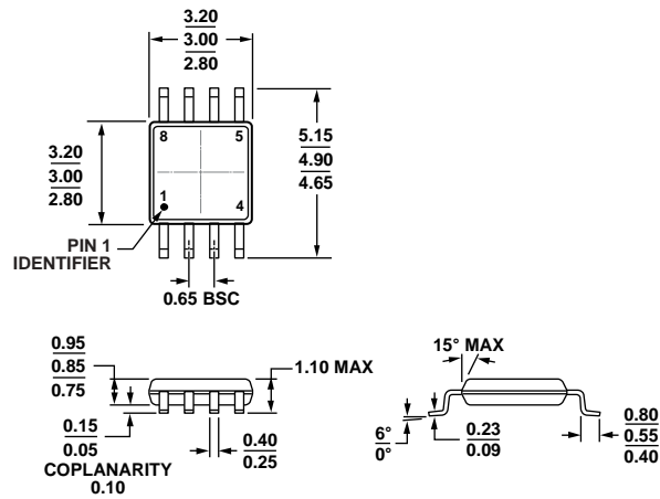
Figure 79. 8-Lead Mini Small Outline Package [MSOP] (RM-8)
