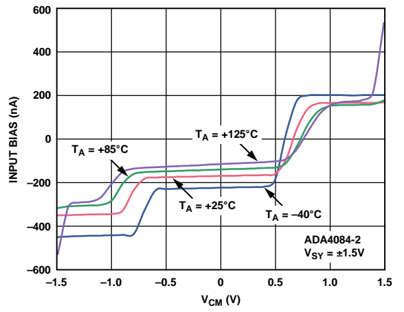
Figure 8. Input Bias Current vs. V_{CM} and Temperature
