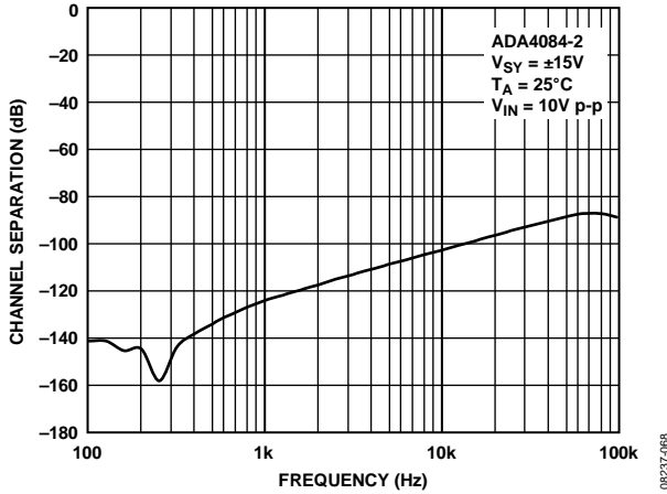
Figure 68. Channel Separation
