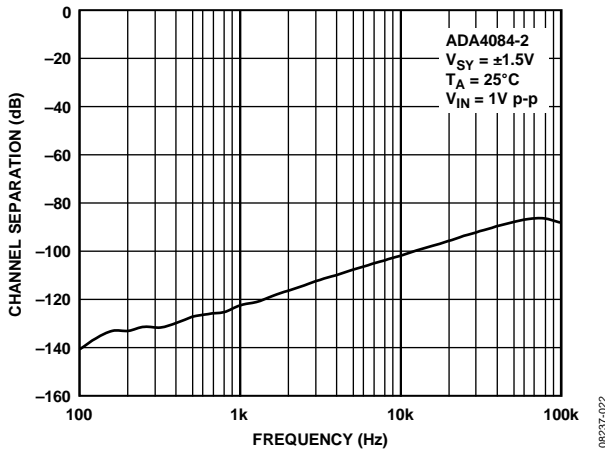
Figure 22. Channel Separation
