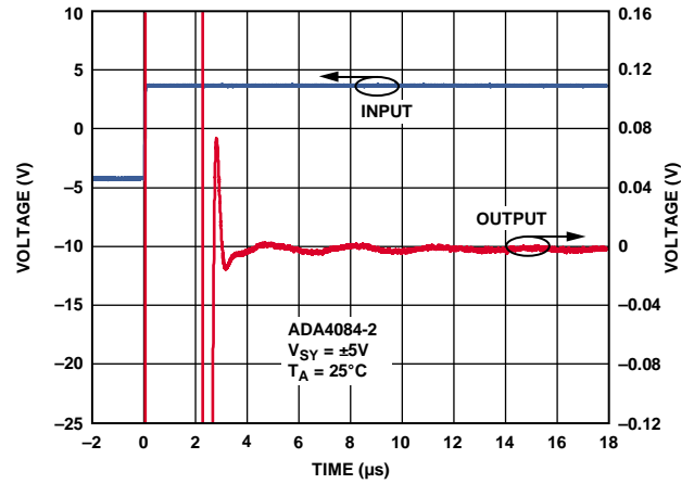
Figure 41. Settling Time
