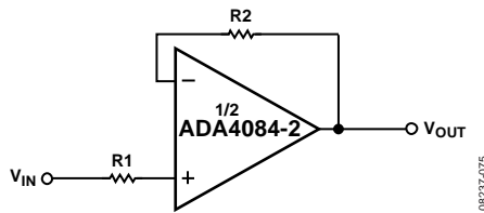
Figure 75. Resistance in Series with Input Limits Overvoltage Currents to Safe Values
