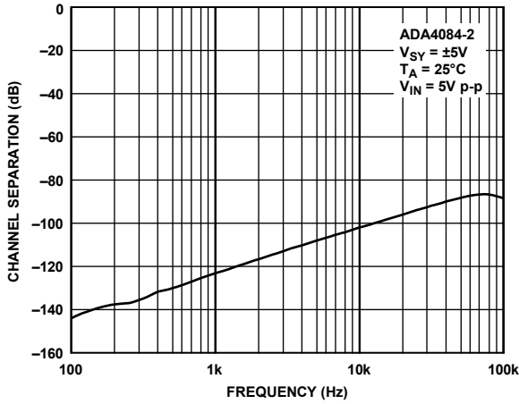
Figure 45. Channel Separation
