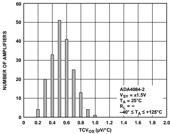
Figure 5. TCV_{OS} Distribution, SOIC
