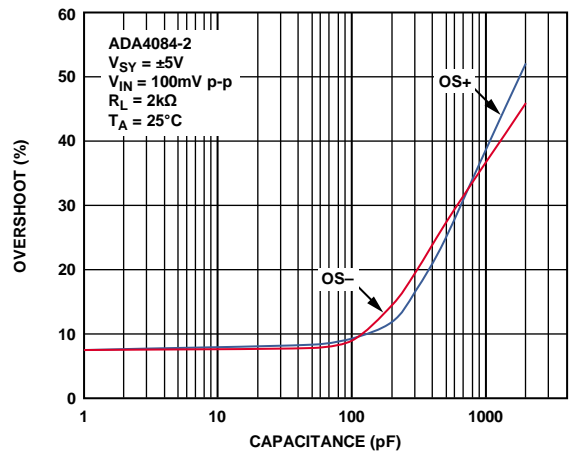
Figure 43. Overshoot vs. Load Capacitance
