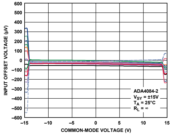
Figure 52. Input Offset Voltage vs. Common-Mode Voltage
