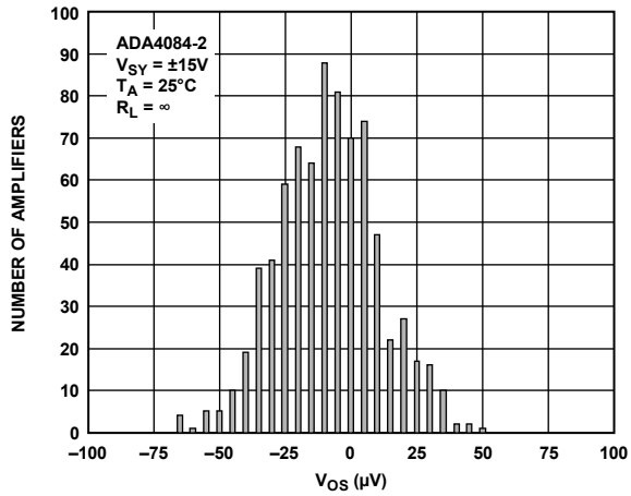
Figure 49. Input Offset Voltage Distribution, SOIC
