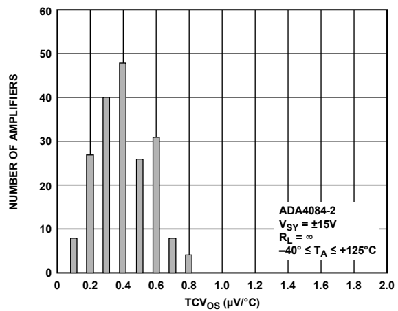
Figure 51. TCV 0s Distribution
