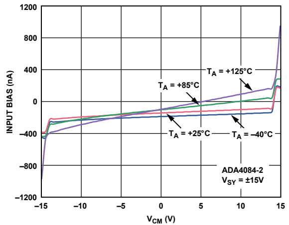
Figure 54. Input Bias Current vs. V_{CM} and Temperature
