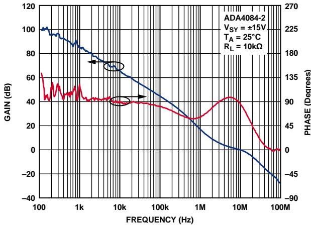
Figure 57. Open-Loop Gain and Phase vs. Frequency
