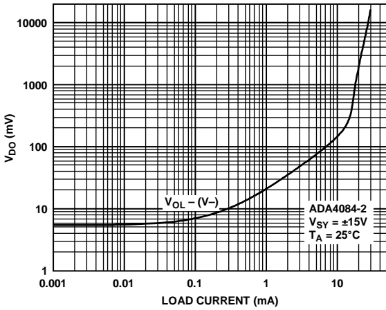
Figure 56. Dropout Voltage vs. Sink Current
