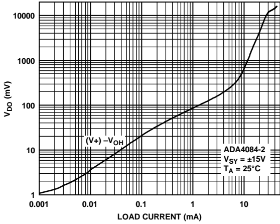
Figure 55. Dropout Voltage vs. Source Current
