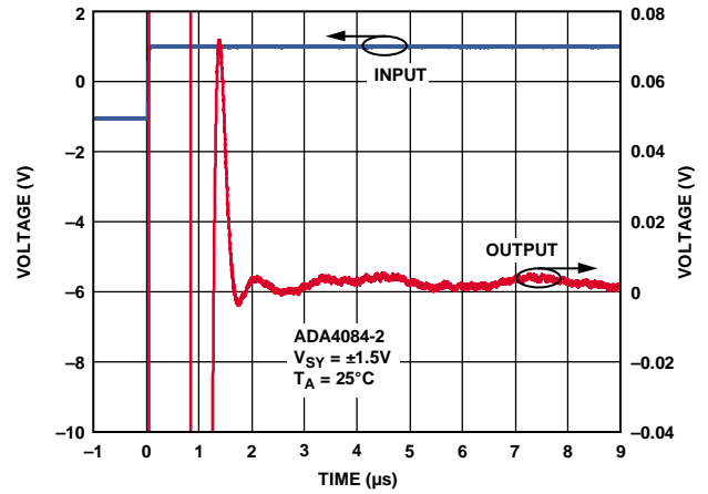
Figure 18. Settling Time
