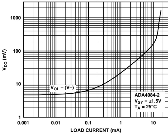
Figure 10. Dropout Voltage vs. Sink Current
