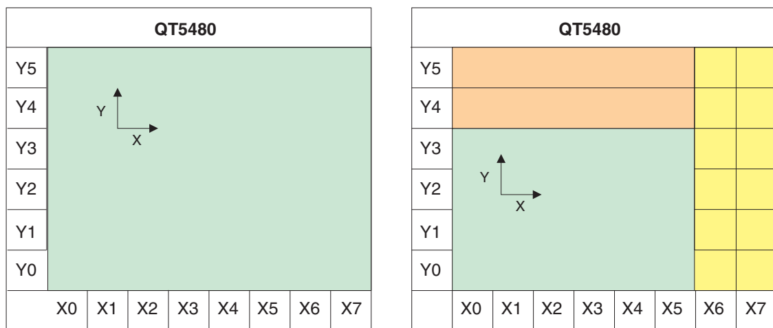
Figure 2-1. Example Touchscreen Configurations
