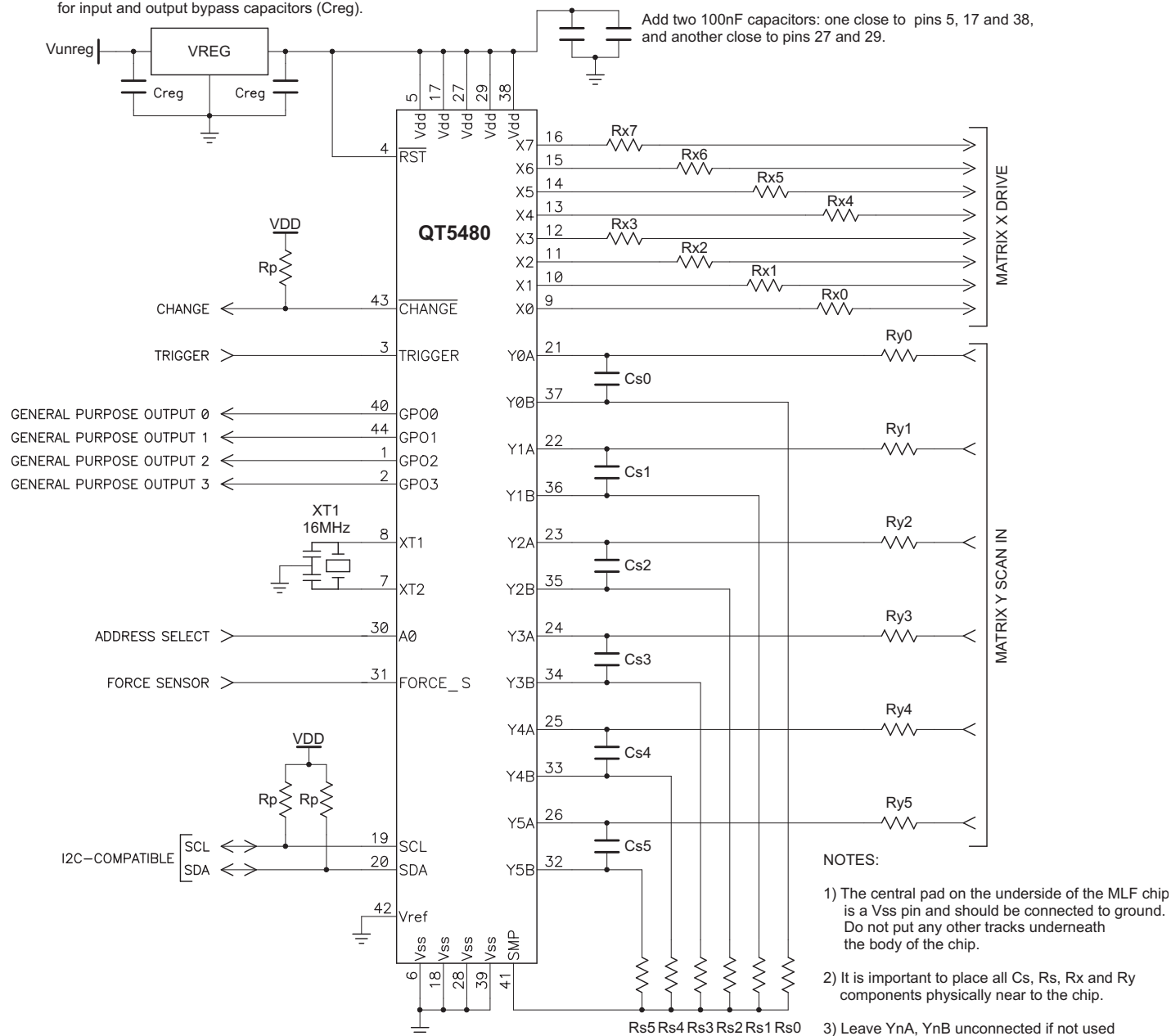
Figure 1-1. Typical Circuit
