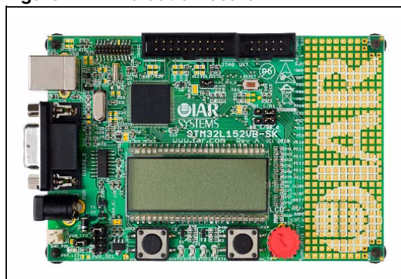
Figure 1. Evaluation board
