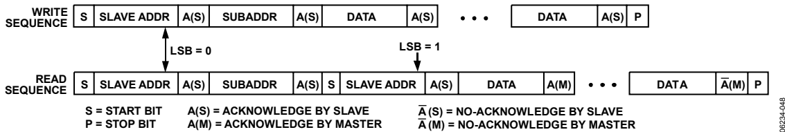
Figure 48. I 2 C Read and Write Sequence
