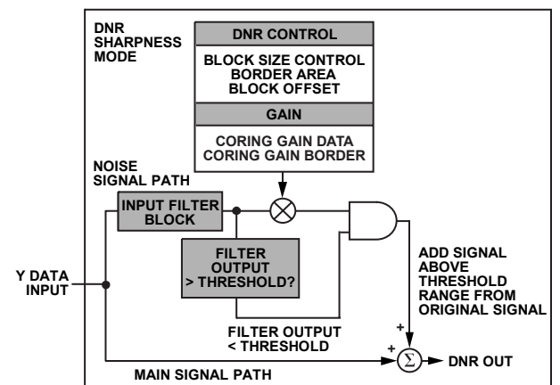
Figure 79. SD DNR Block Diagram
