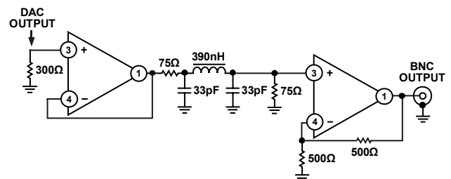
Figure 88. Example of Output Filter for HD, 4 \times Oversampling
