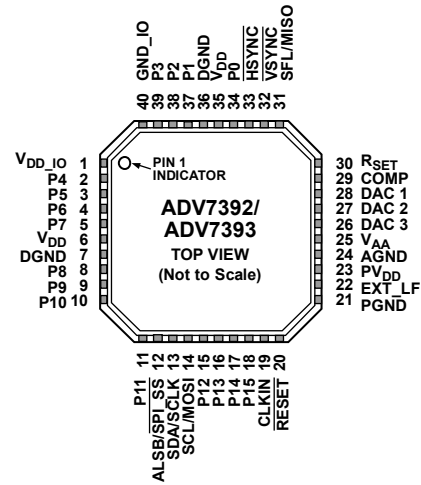
Figure 18. ADV7392/ADV7393 Pin Configuration
