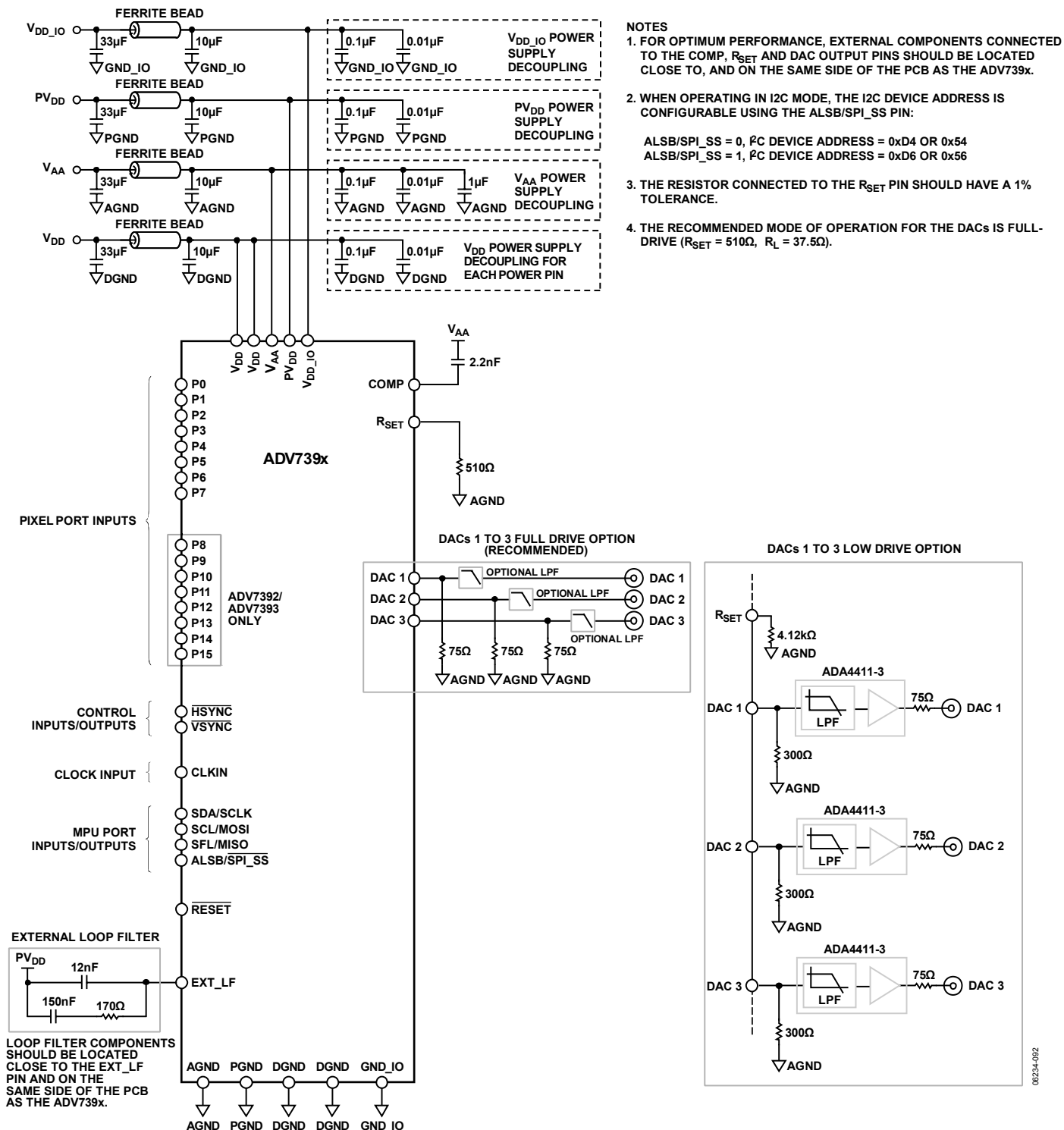
Figure 92. ADV739x Typical Application Circuit
