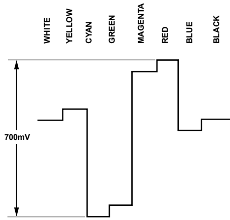
Figure 117. Pr Levels—NTSC
