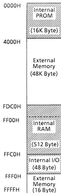
TMP90PH02 Memory Map
