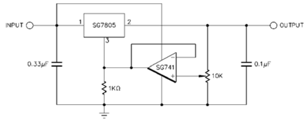
Figure 8 – Adjustable Output Regulator, 7V to 30V
