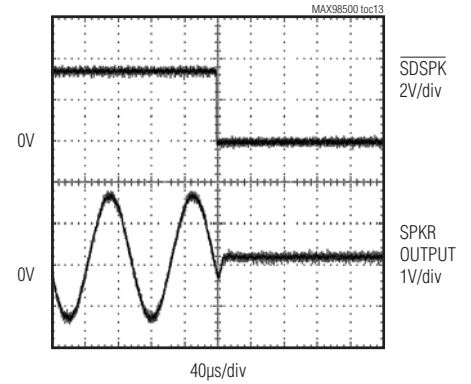
SHUTDOWN RESPONSE
