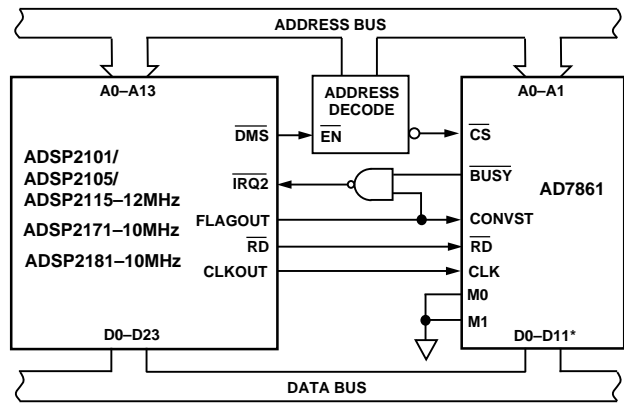
Figure 5. ADI Digital Signal Processor/Microcomputer Interface
