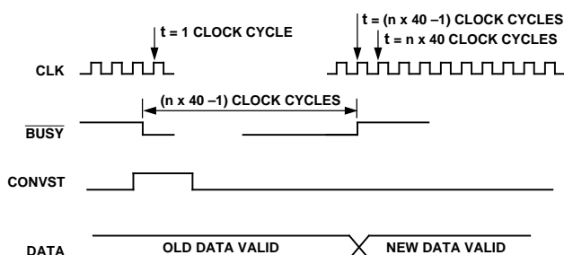
Figure 3. Busy Pulse Timing
