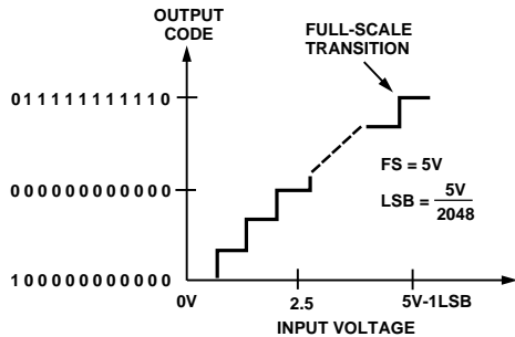
Figure 4. AD7861 Transfer Function
