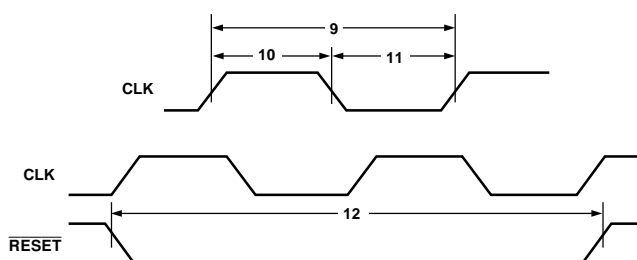
Figure 2. Write Cycle Timing Diagram
