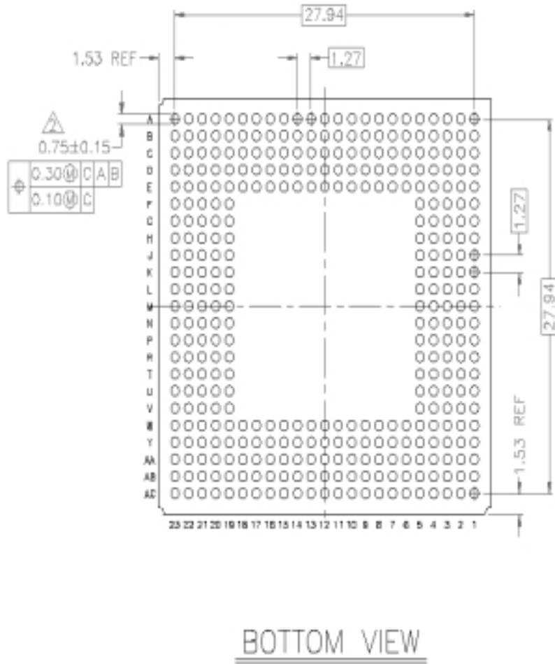
Figure 2-3: Pin Location and Signal Cross-References (Bottom View)
