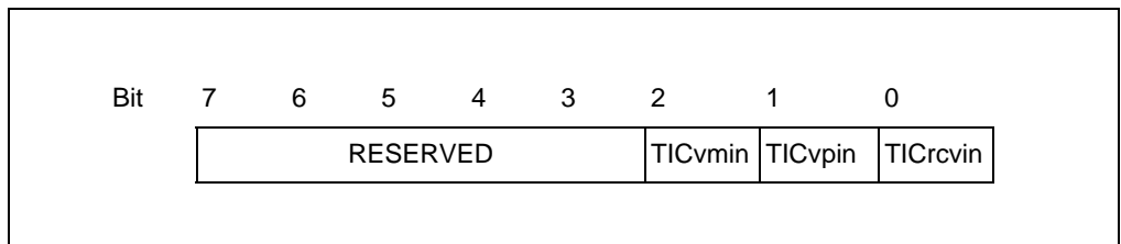
Figure 12-28: Input TIC register for TIC mode
