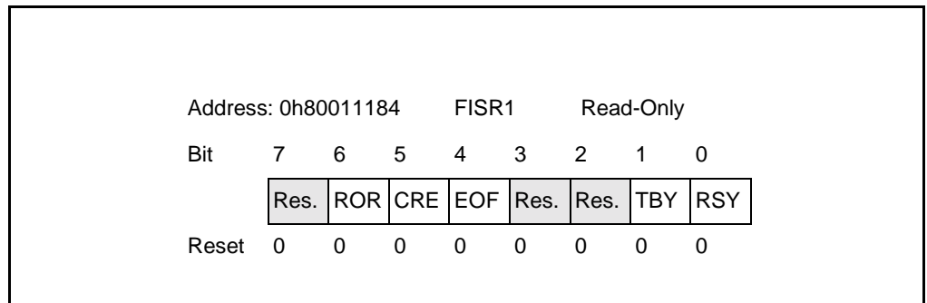
Figure 12-15: Flr status register 1 bits
