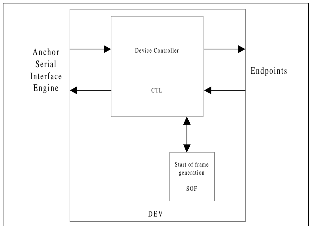
Figure 12-18: Device Interface
