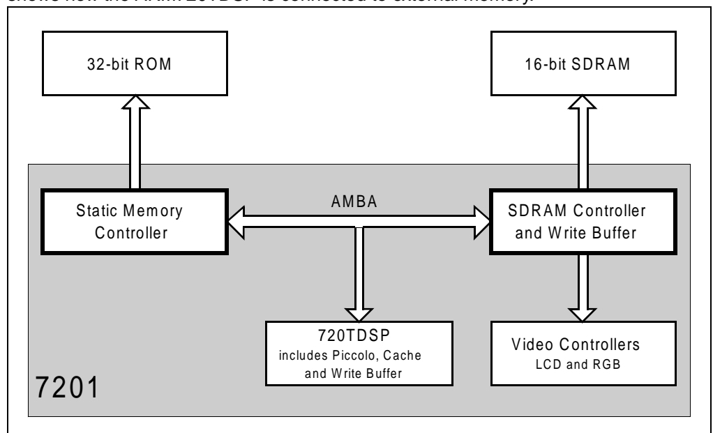
Figure 5-2: ARM720TDSP Connected to External Memory
