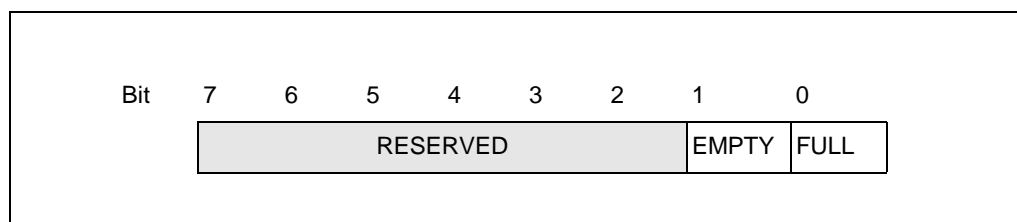
Figure 12-24: USBD Status Register Bits
