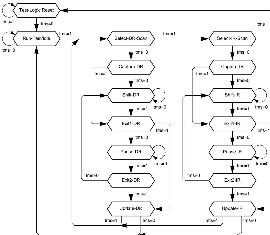
Figure 14-1: Test Access Port (TAP) Controller State Transitions
