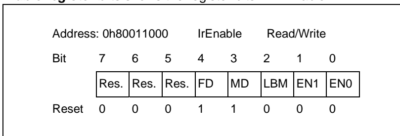
Figure 12-2: Ir Enable register bits
