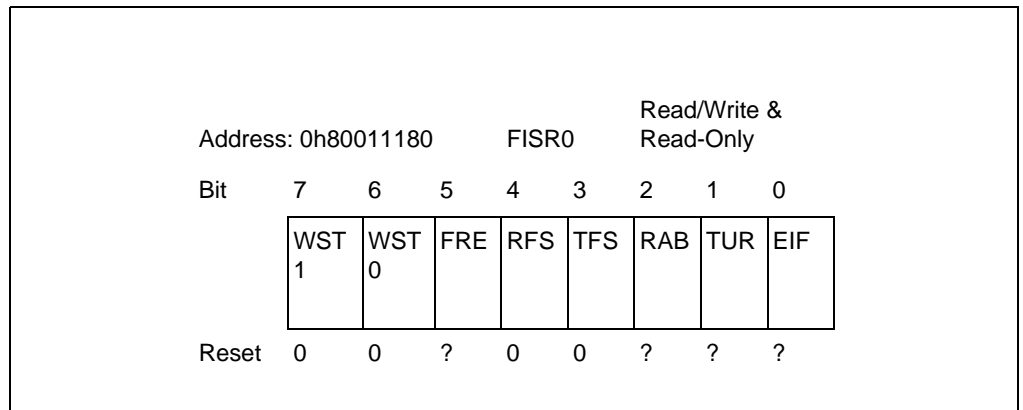
Figure 12-14: Flr status register 0 bit locations
