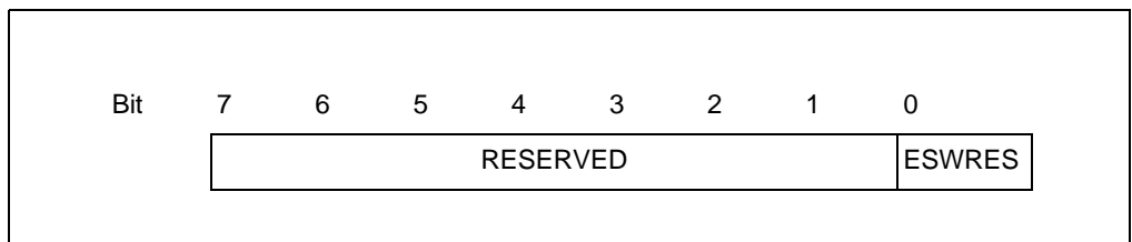
Figure 12-30: Generate software reset to USBD
