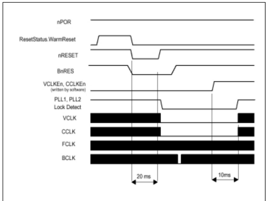
Figure 7-4: Software Generated Warm Reset
