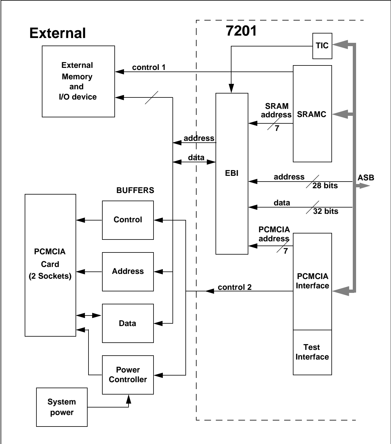
Figure 10-1: Overview of External Memory and Static Memory Control
