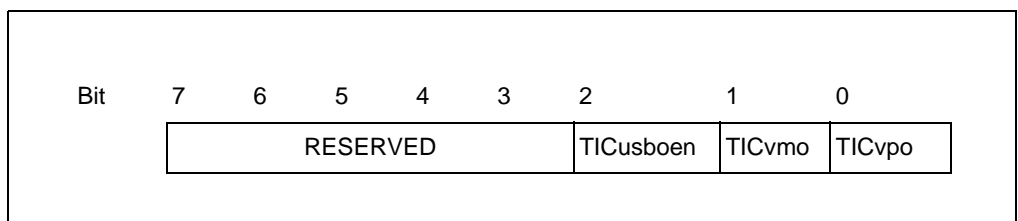
Figure 12-29: Output TIC Register for TIC mode
