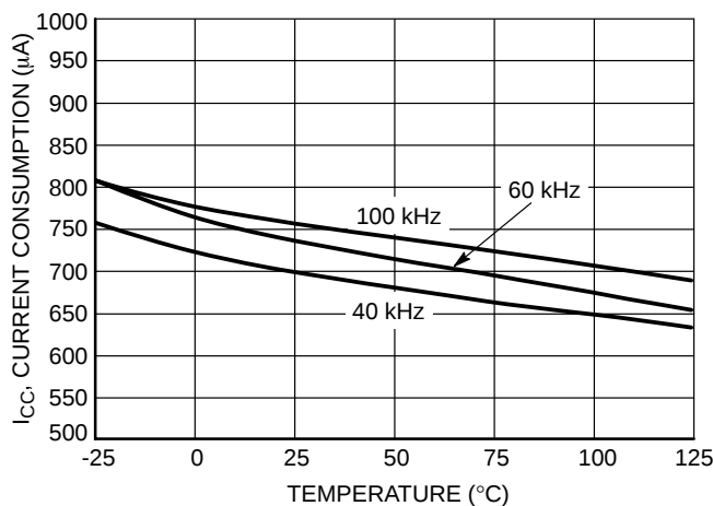
Figure 5. I_C Current Consumption (No Load) versus Temperature
