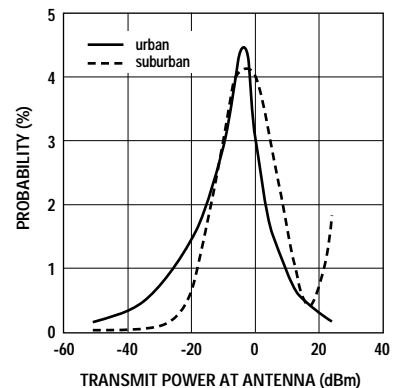
Figure 34. Probability Distribution of Mobile Transmit Power.
