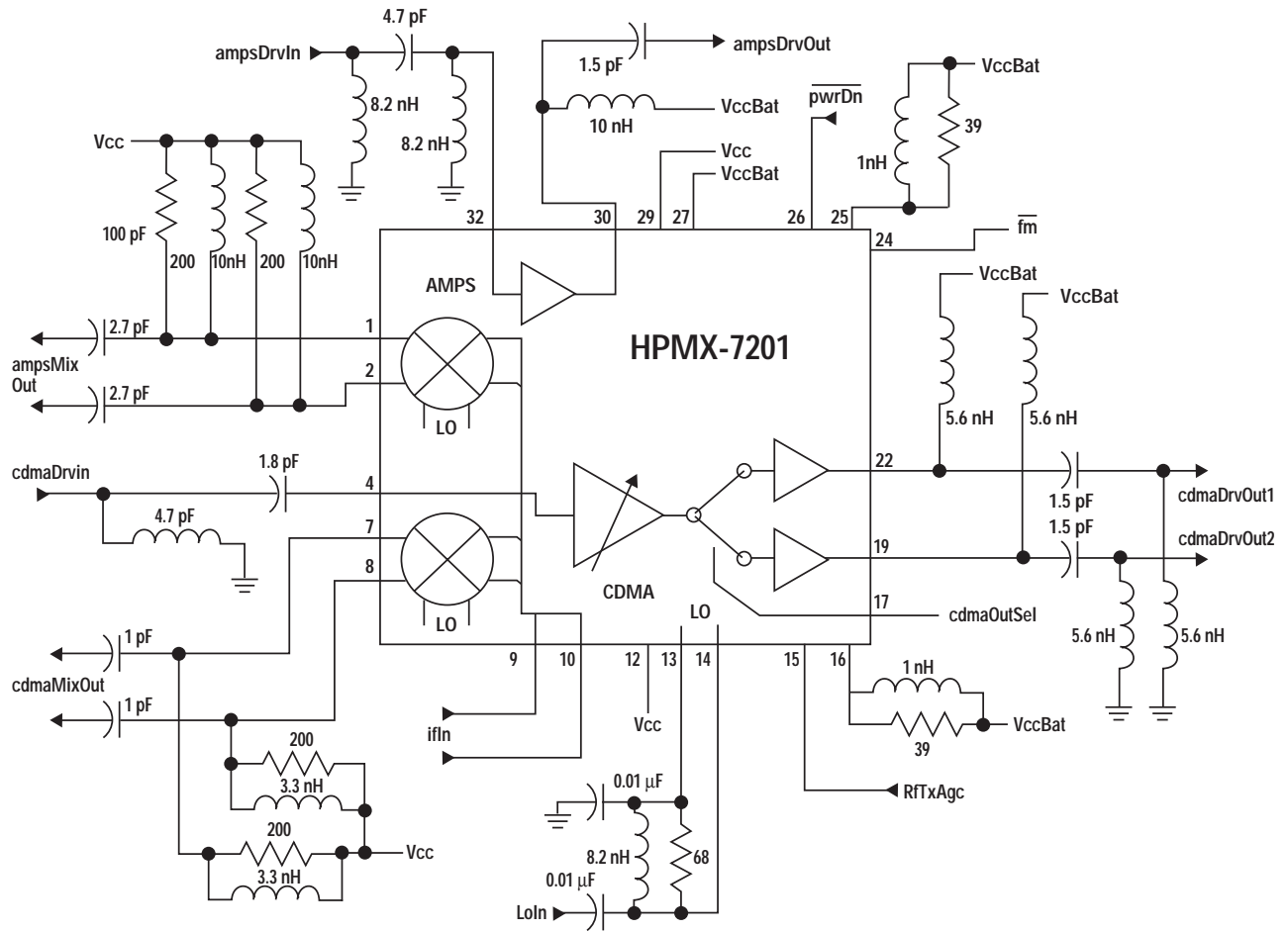
Figure 31. Example Reference Circuit for the HPMX-7201.
