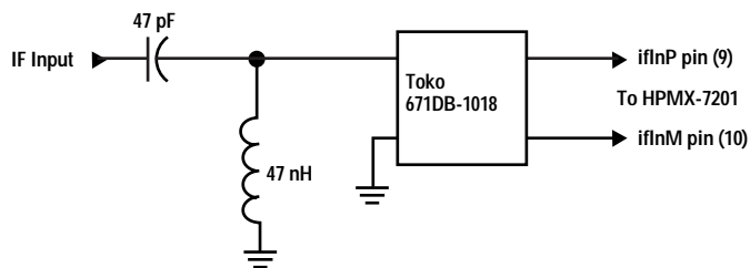
Figure 32. Test Circuit for Single-ended 50Ω IF Operation.
