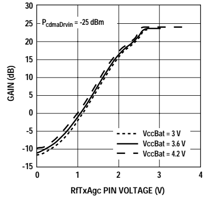
Figure 9. CDMA Driver Gain vs. V(RfTxAgc) and VccBat.
