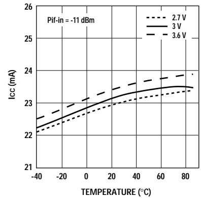
Figure 15. AMPS Upconverter Icc vs. Temperature and Vcc.
