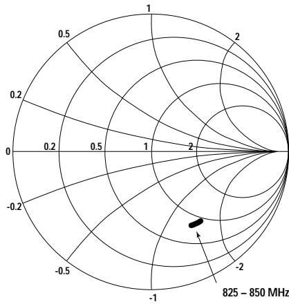
Figure 28. ampsDrvOut Output Impedance vs. Frequency.
