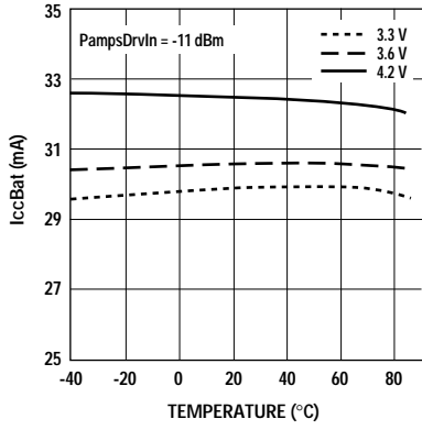
Figure 19. AMPS Driver IccBat vs. Temperature and VccBat.
