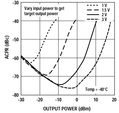
Figure 12. CDMA Driver ACPR vs. Output Power and V(RfTxAgc).
