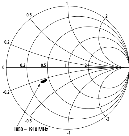
Figure 26. cdmaDrvOut Output Impedance vs. Frequency.
