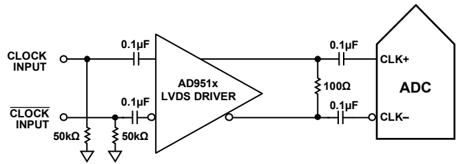
Figure 66. Differential LVDS Sample Clock (Up to 1 GHz)
