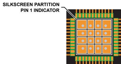
Figure 75. Typical PCB Layout
