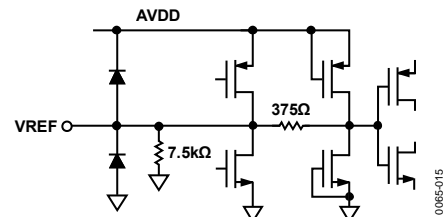
Figure 54. Equivalent VREF Circuit
