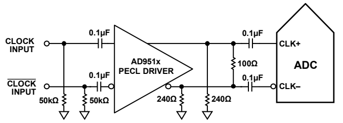
Figure 65. Differential PECL Sample Clock (Up to 1 GHz)
