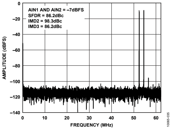
Figure 37. Two-Tone 16k FFT with f_{IN1} = 70.5 \text{ MHz} and f_{IN2} = 72.5 \text{ MHz} , f_{SAMPLE} = 125 \text{ MSPS}
