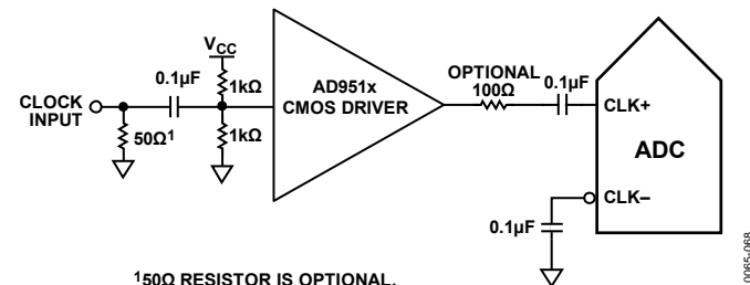
150Ω RESISTOR IS OPTIONAL. Figure 67. Single-Ended 1.8V CMOS Input Clock (Up to 200 MHz)
