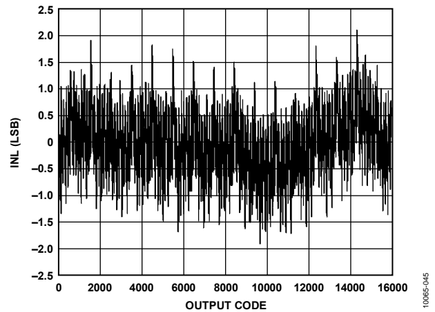
Figure 41. INL, f_{IN} = 9.7 \text{ MHz} , f_{SAMPLE} = 125 \text{ MSPS}
