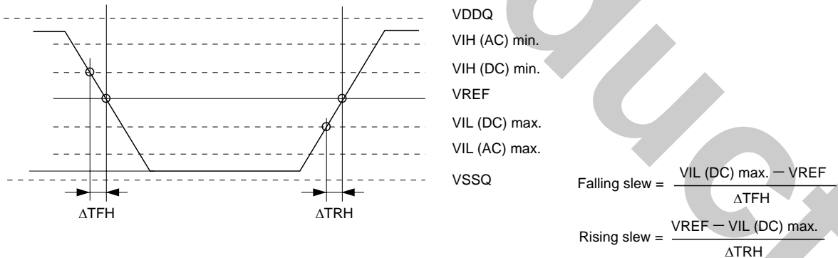
Input Nominal Slew Rate Definition for Single-Ended Signals
