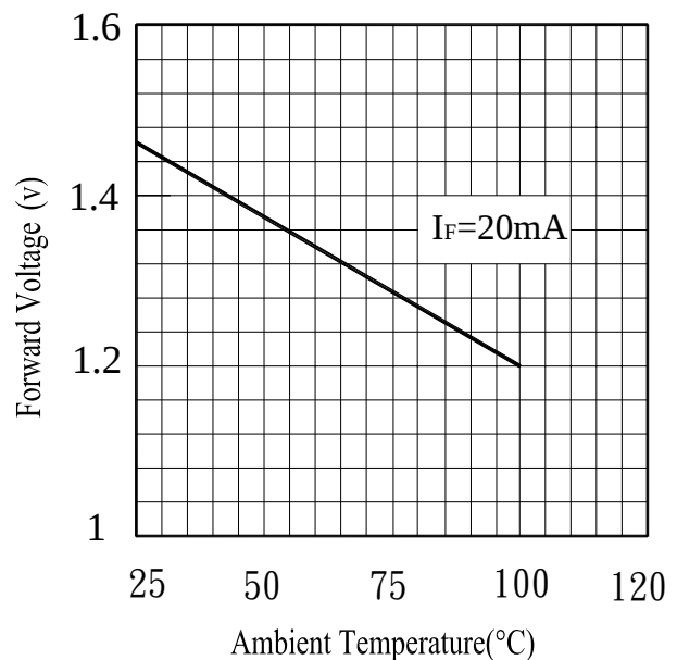
Fig.8 Forward Voltage vs.
