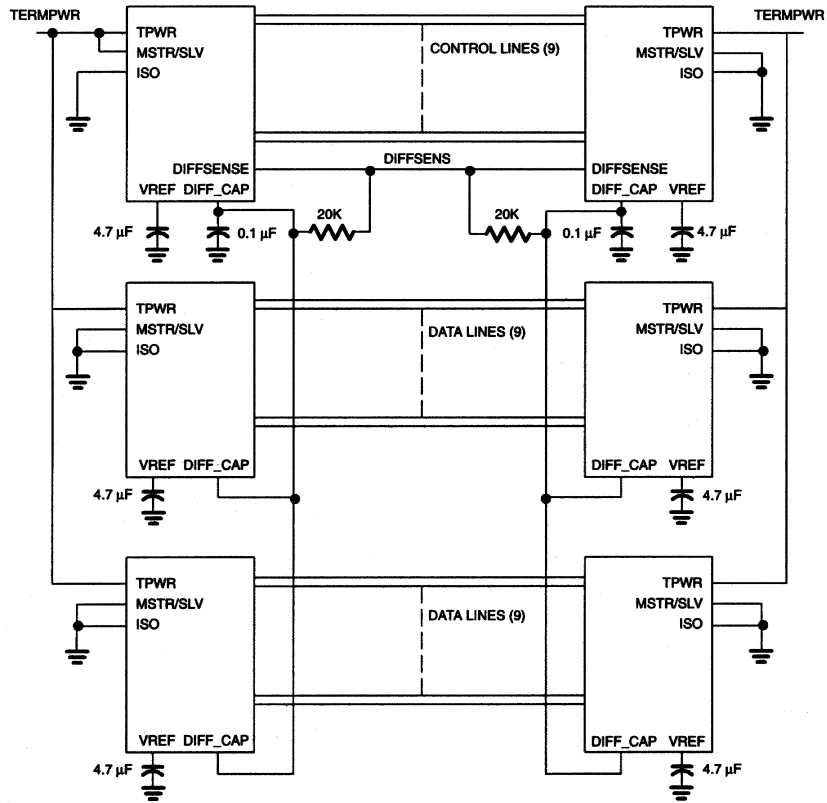
SCSI BUS CONFIGURATION Figure 2
