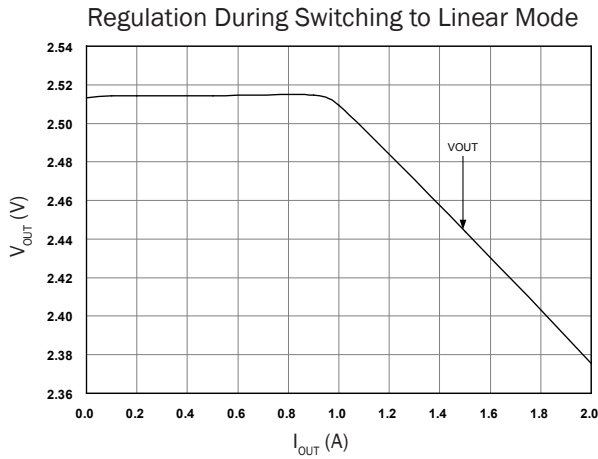
Figure 13. Loading Regulation
