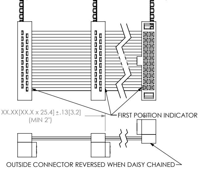
FIG. 4 (FFSD-10-D-XX.XX-01-X-N-DXX-O SHOWN) (SAME AS FIG. 1, DIFFERENT AS SHOWN) (2.00[50.8] MINIMUM, 1.00[25.4] INCREMENTS)
