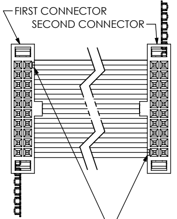
(FFSD-10-D-XX.XX-01-X-N-RN2 SHOWN) (SAME AS FIG. 1, DIFFERENT AS SHOWN)
