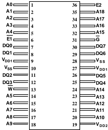
Figure 2. 10ns SRAM Pinout (36)
