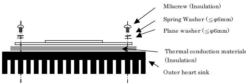
Recommended installation screw pitch
